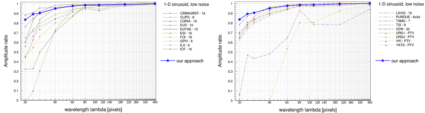
Fig. 13. Synthetic vector field, PIV-Challenge 2005, Case A4, region Sinusoids II : Part 1 and 2 of the comparison of the amplitude response depending on the structure wavelength \lambda . We included the measurement of our experiments into the plot hard-copied from [28, Fig. 21a] (we redraw the numbers of the horizontal axis for better readability) where 19 flow measurement implementations were compared. Most approaches use cross-correlation while the methods labelled by CLIPS-8 and CEMAGREF-16 are based on optical flow. ESI and *-PTV are particle tracking velocimetry methods. For a description of the competing approaches we refer to [28]. Our approach outperforms most of the other implementations, especially the accuracy for very small structures was improved by using adaptive windows.
