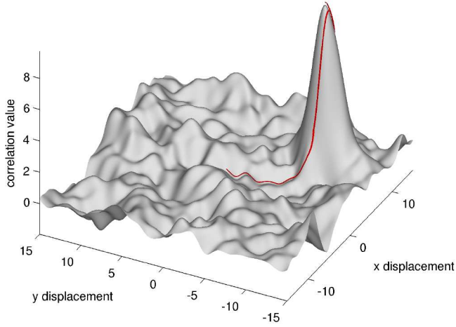
Fig. 4. Value of the cross-correlation-function, -C(u, \Sigma, x) between two particle images and a path (starting in (0, 0) ) of a gradient-based optimisation approach. Multiscale techniques are employed to avoid that the process stops in a local optimum and to find the correlation peak in (8, -8) .
