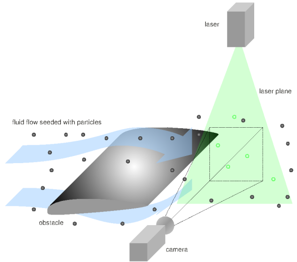
Fig. 1. Particle Image Velocimetry (PIV) experimental setup: The flow of a fluid behind an obstacle shall be examined. To this end, it is seeded with small particles. A laser projects a thin plane into the region of interest and illuminates the particles therein. Fluid motion can be measured by analysing the image sequence recorded by a camera system.
