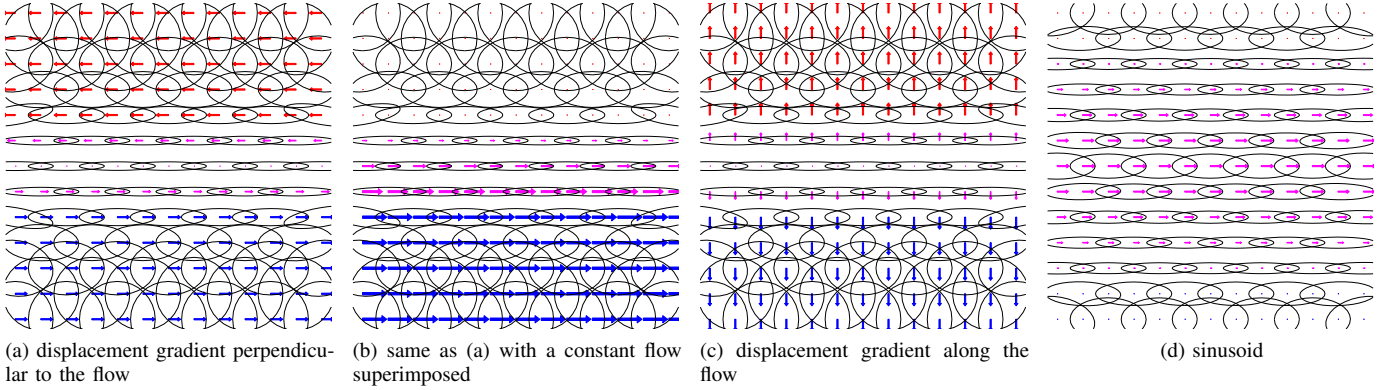
Fig. 9. Synthetic displacement fields (arrows) and some of the adapted windows (ellipses). Constant vector fields (upper and lower region) enclose a transition zone (middle). Affine transition zone: Identical window shapes for different vector fields: (a) displacement gradients perpendicular to the flow, (b) superimposed by a constant field, and (c) gradients parallel to flow. Sinusoid: (d) Transition zone is sinus-shaped ([0, \pi]) . The adaptation scheme aligns the windows perpendicular to the displacement gradient and reduces the size along the transition direction to avoid smoothing out the boundary.
