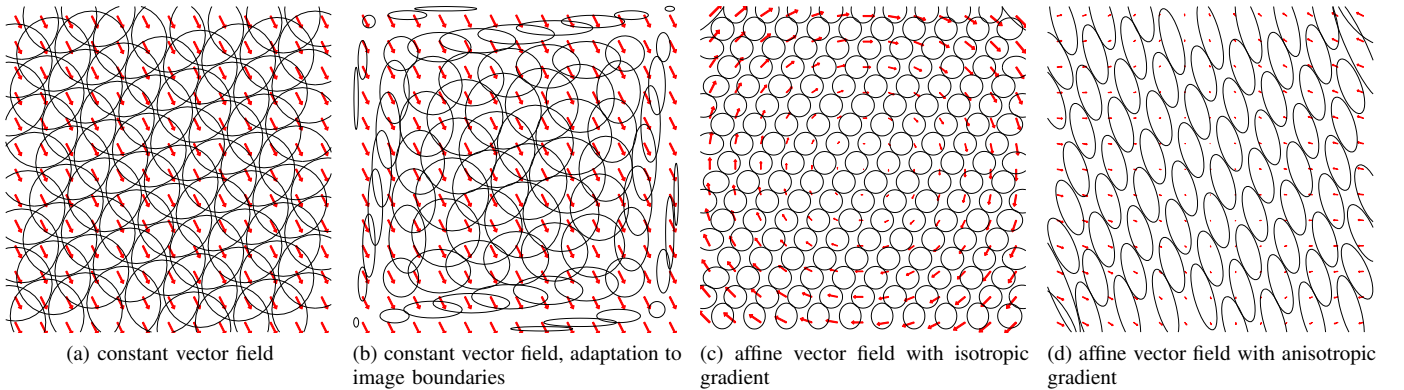
Fig. 8. Synthetic displacement fields (arrows) and some of the adapted windows (ellipses). Constant vector fields: (a) The window radii would approach infinity due to the lack of a gradient, but is limited by the constraint r \leq 6 . (b) The windows are additionally constrained to adapt to the boundaries of the image domain by setting e_{\text{outside}} = 10 . Affine vector fields: (c) Rotational field with isotropic gradients leads to round windows. (d) Vector field with anisotropic gradients leads to ellipse-shaped windows.
