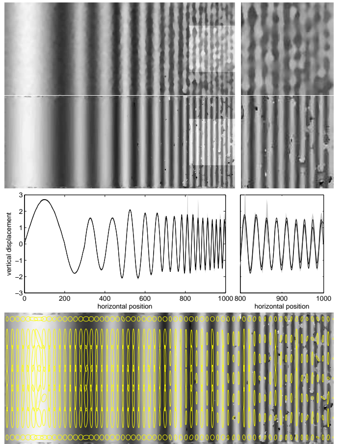
Fig. 12. Synthetic vector field, PIV-Challenge 2005, Case A4, Sinusoids II (with additive image noise and unpaired particles), full and detailed view of the estimated vertical displacement component (colour map identical to Fig. 6): Row 1: The high amount of image noise necessitates large windows ( r = 8 ) for the approach based on fixed windows. Thus, details are smoothed out, but the general structures can be resolved. Row 2: Using the previous result as initialisation, joint correlation and window adaptation ( \sigma = 40 ) can significantly improve the accuracy even for the smallest structures, however interrupted by local outliers. Row 3: statistics (along the complete vertical axis, but 10 px excluded at the upper and lower boundary) of the results in row 2: mean displacement (thick line), range of \pm one standard deviation (shaded gray) and ground truth (thin line, cf. Fig. 6c), Row 4: The windows align perpendicular to the gradient with exception of the vicinity of outliers.
