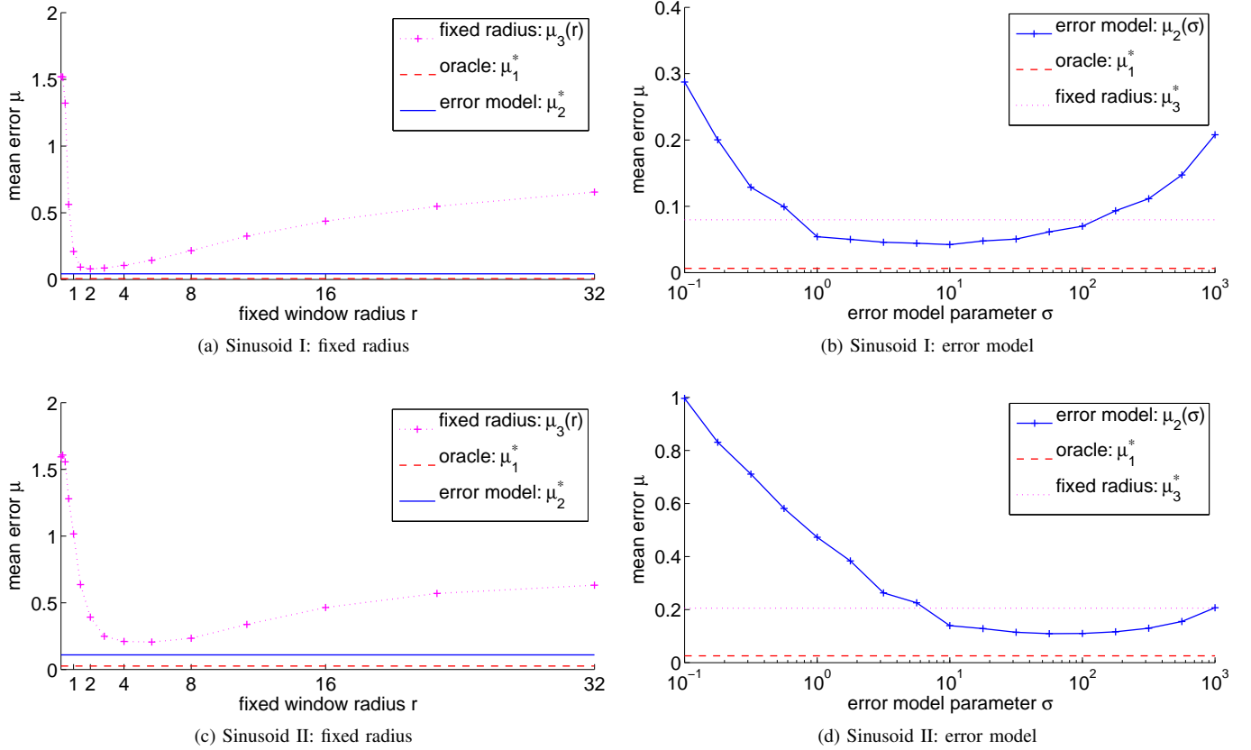
Fig. 7. Comparison of window selection strategies: mean error of the fixed radius (dotted line), oracle (dashed line) and the error model based strategy (solid line). (a) Results for Sinusoids I , comparing the fixed radius \mu_3(r) strategy for varying radii to the best values of the alternative strategies. (b) Same as (a), but for the error model strategy and varying parameter \sigma . Best results are \mu_1^* = 0.00627 , \mu_2^* = 0.0421 (for \sigma^* = 10 ) and \mu_3^* = 0.0796 ( r^* = 2 ). (c)-(d): Same as (a)-(b), but for the data set Sinusoids II , with \mu_1^* = 0.0255 , \mu_2^* = 0.109 ( \sigma^* = 10^{7/4} ), \mu_3^* = 0.206 ( r^* = 2^{5/2} ).
