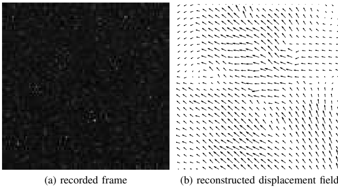
Fig. 2. Particle Image Velocimetry (PIV): (a) Detail of an image frame recorded in a real fluid experiment (see Sect. IV-D), showing particles (polyglycol diluted in water) in an air flow. The image is 100 \text{ px} \times 100 \text{ px} in size, corresponding to 7.5 \text{ mm} \times 7.5 \text{ mm} in the illuminated plane. The particles have a diameter of less than 10 \mu\text{m} i.e. less than a pixel in the projection, which prevents the application of standard differential optical flow techniques. Image noise level is high. (b) Example of a reconstructed displacement field. Each arrow describes the motion vector estimated at its origin.
