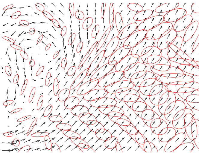
Fig. 3. Estimated displacement field in a real turbulent PIV experiment (arrows) and some of the adapted correlation windows (represented by ellipse-shaped level contours). For each measurement, our approach balances the error caused by a high amount of image noise compared to the supporting region, and violation of the assumption, that the flow is constant within the window, such as in the upper left region, where high gradients dominate. In contrast, windows can be chosen larger in homogeneous regions (right). This spatially-dependent adaptivity of windows emerges from our variational approach.
