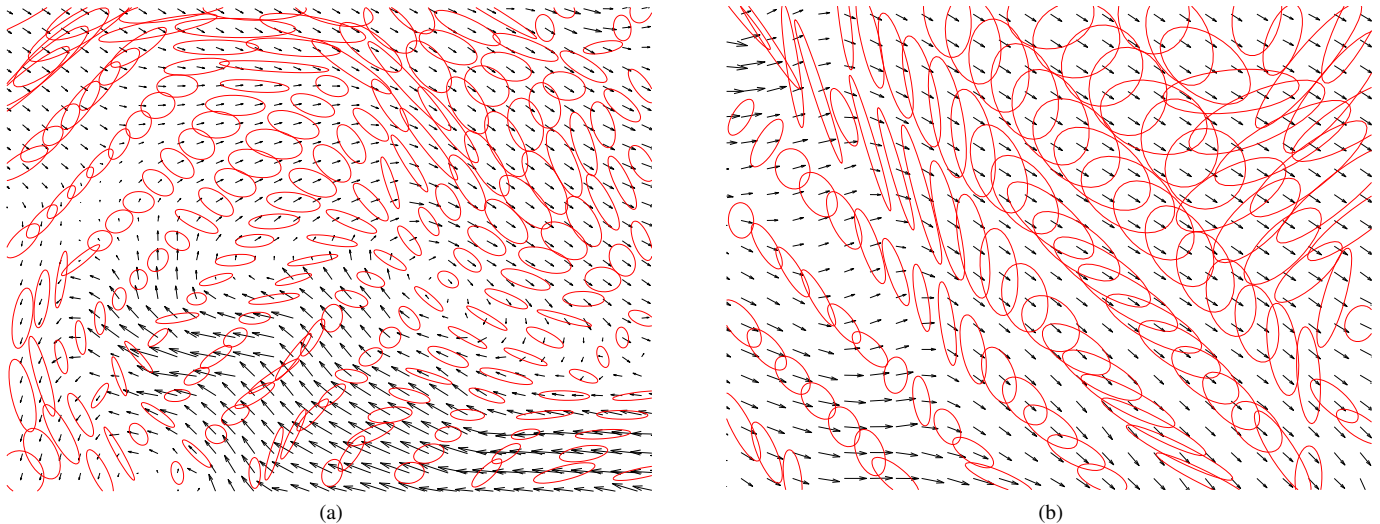
Fig. 16. Real 2D PIV experiment: Detailed views of Fig. 14, showing the estimated displacements (arrows) and adapted windows (ellipses). (a) In the vicinity of a complex flow, the ability to adapt the window orientation continuously proves beneficial. (b) Windows orientations do not necessarily coincide with the direction of the flow, but are perpendicular to the velocity gradient here (upper left).
